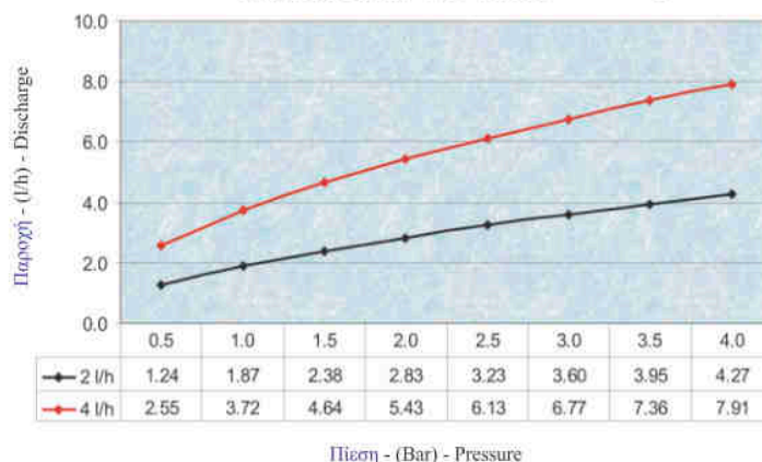
Paladrip 16mm - 2 &amp; 4 LPH
