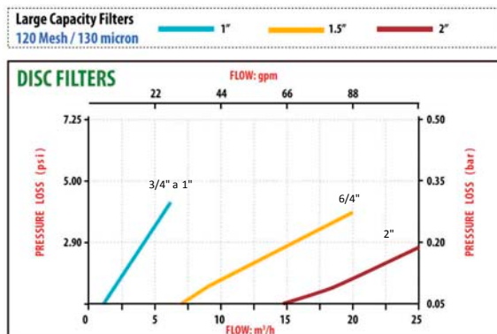
Disc &amp; Screen Filters
